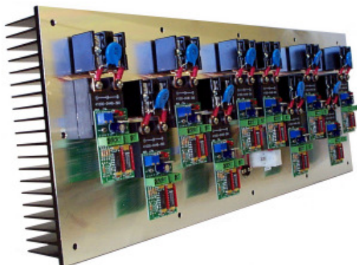
Example of an external mount controller
